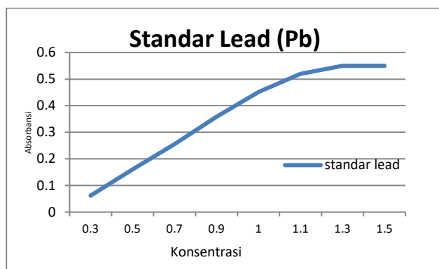
Gambar 2.1 Kurva Standar Lead Pb (Timbal)
