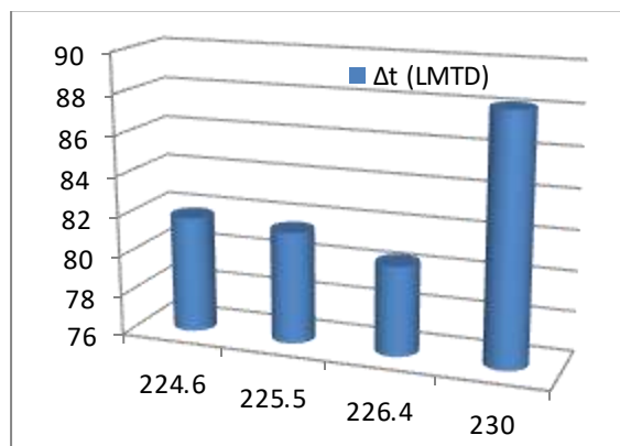
Gambar 2. Grafik Perbandingan Temperature Inlet Steam Terhadap \Delta t LMTD
