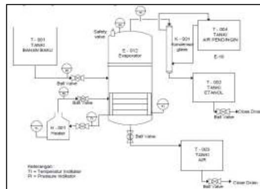
Gambar 1. Alat Evaporator
