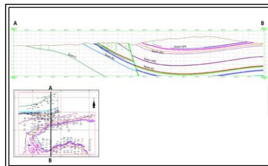
Gambar 3.2 Penampang Melintang Seam
