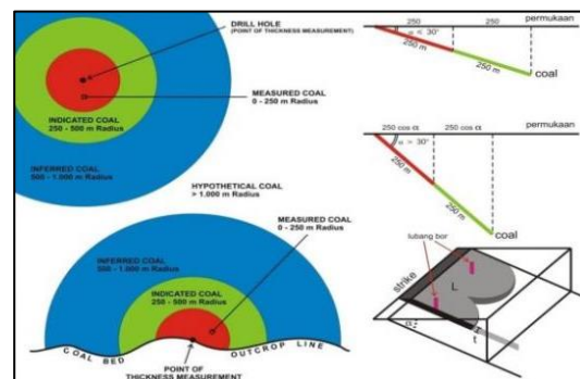
Gambar 3.1 Model Perhitungan Sumberdaya
